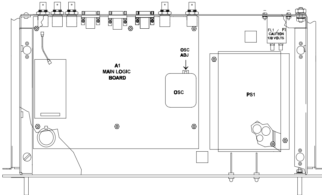
Figure 5-1. Model 8821A-11 Major Assembly Locations
